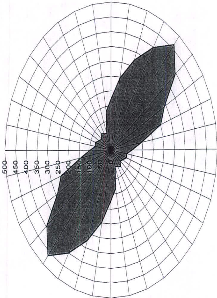
Fig. 7-28 : Rose Diagram of Fault Azimuth Frequency in Jebel-e-Barez 1/100,000 Sheet .
