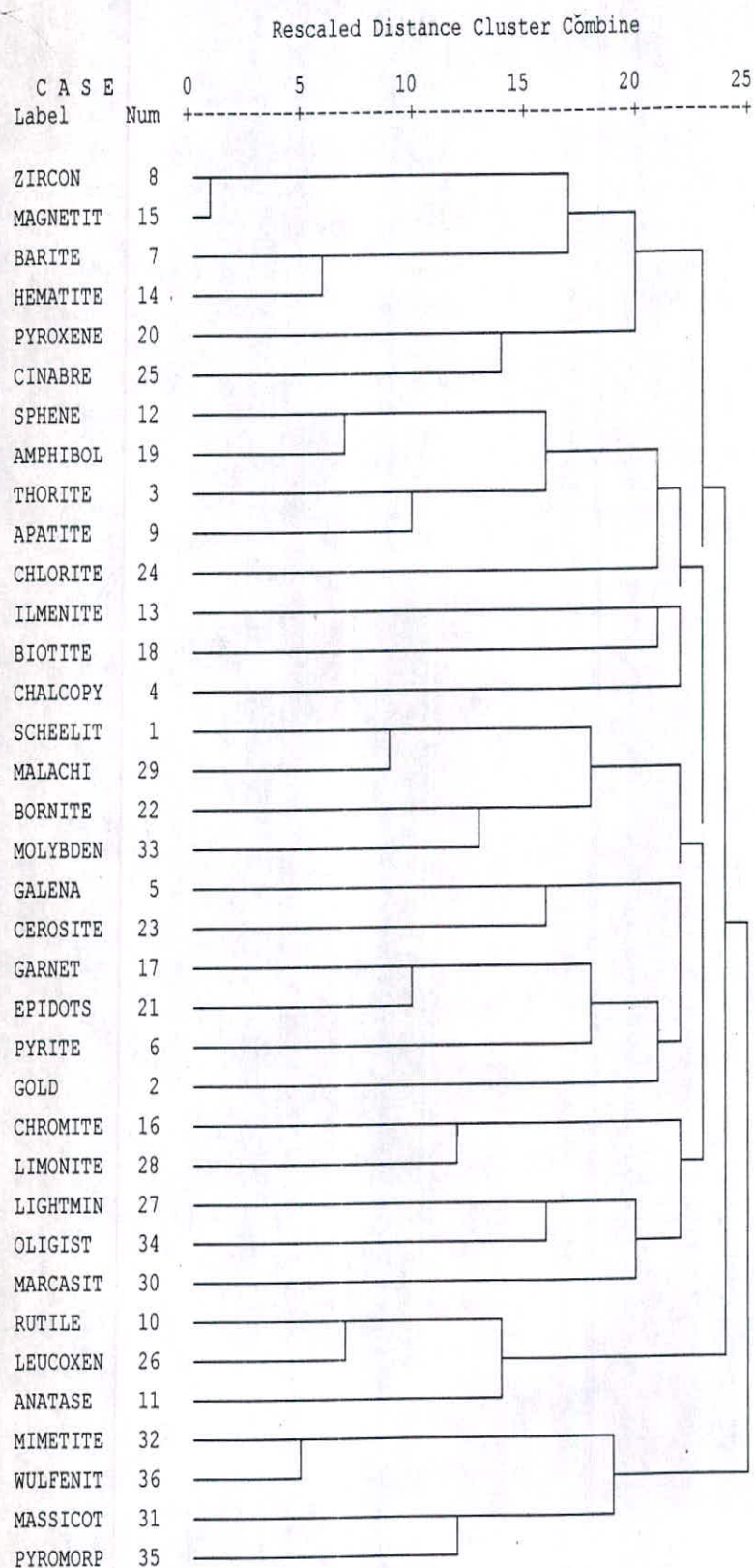
Fig. 7-25 : Dendrogram of Heavy Mineral Variables in JEBAL-e-BAREZ 1/100,000 Sheet .
