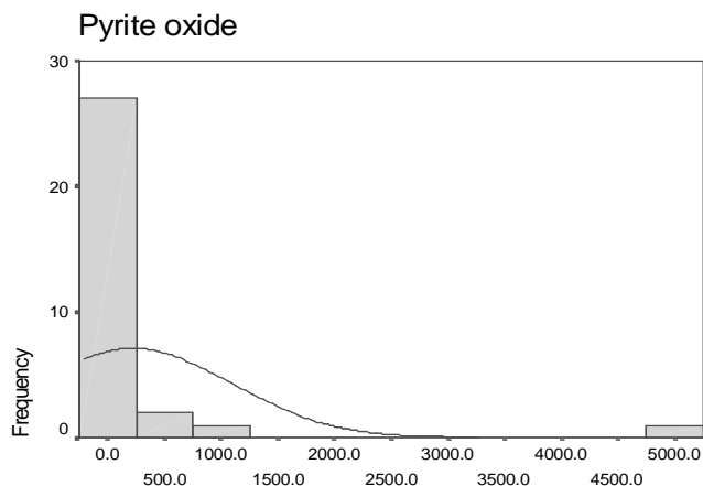
Pyrite oxide
