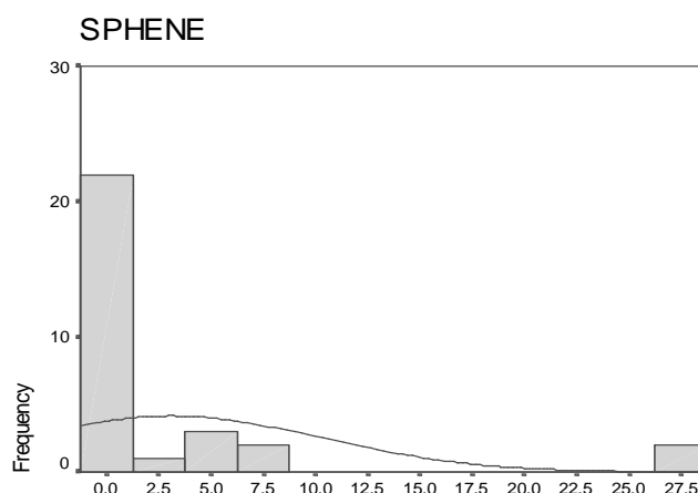
SPHENE
