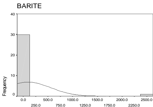
BARITE
