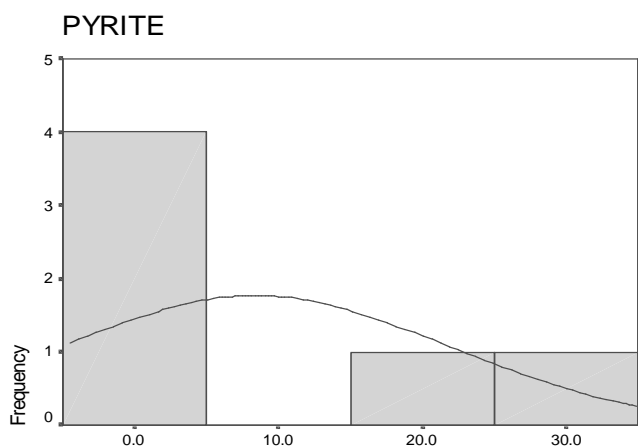
PYRITE
