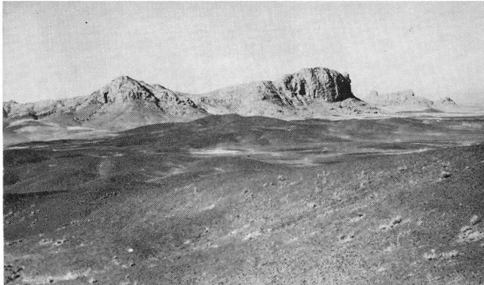
Fig. 4. Kuh-e-Chavosh from south. Cretaceous limestone surrounded by Tertiary andesite. (Photo J. Stocklin.)
