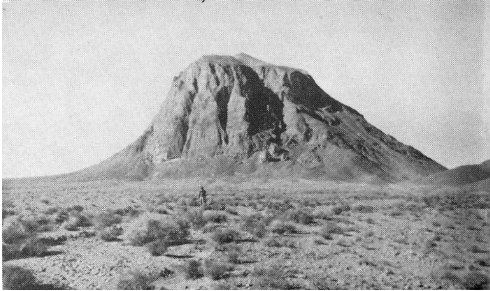
Fig. 7. Mikh-e-Khur, pyroxene andesite. (Photo M.H. Nabavi.)
