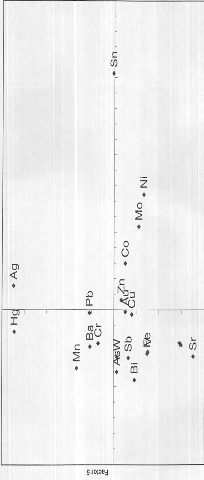
Factor 3 Fig 6-9 :Graphical Representation of Factor Analysis for Geochemical Variables in Sari 1:100,000 Sheet
